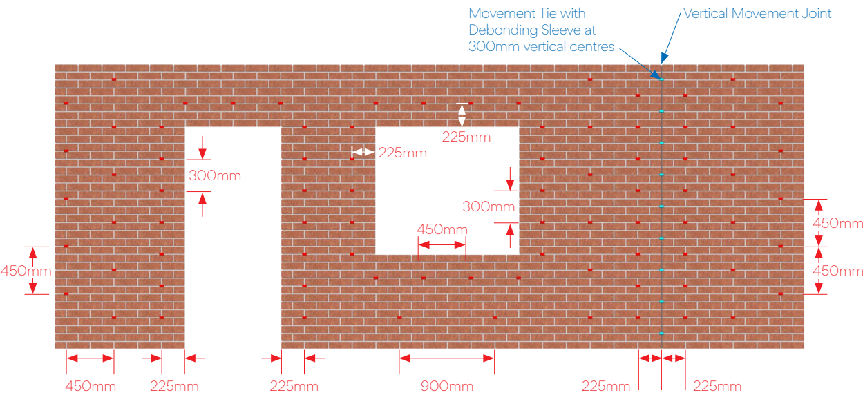
Example of the Tie Positioning required in accordance with PD 6697:2019 and BS 5628-1:1992
